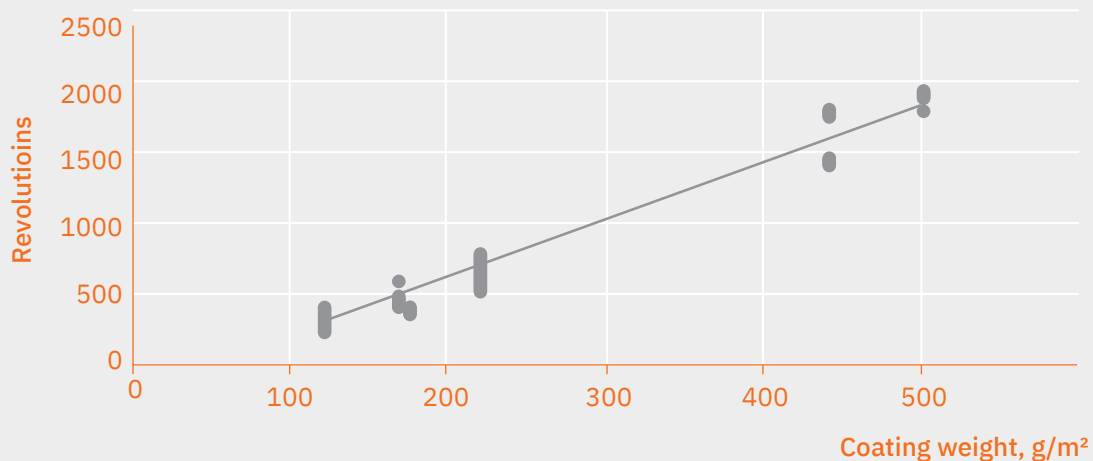
Figure 3.3. Wear resistance of Riga Form plywood
