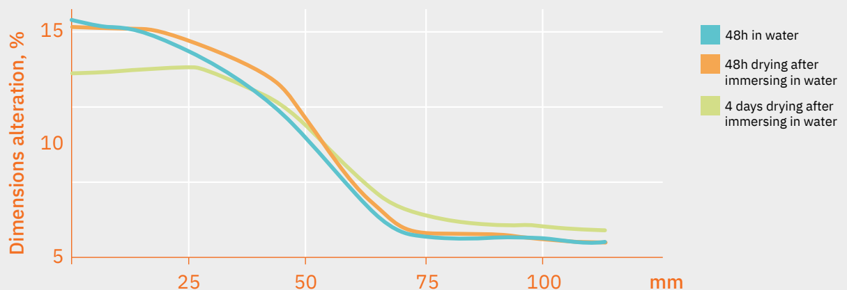
Figure 5.8. Dimension alteration
